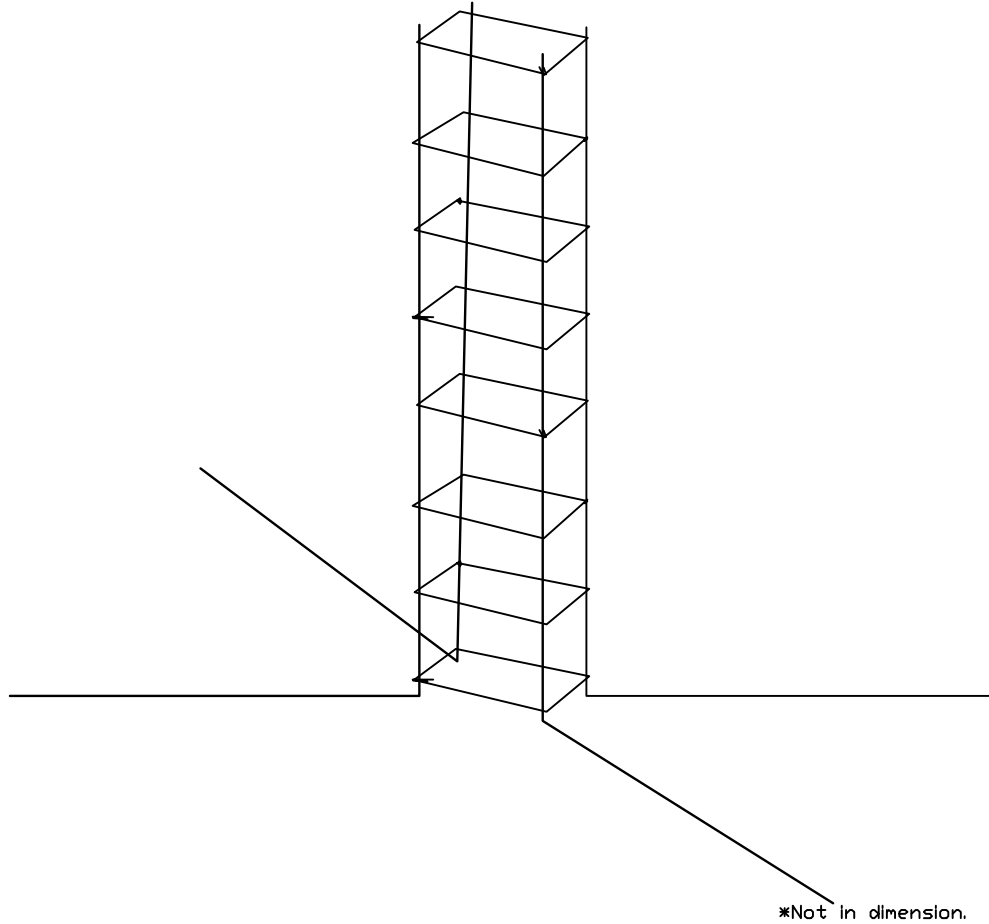
Perspective view: Reinforcement of column
